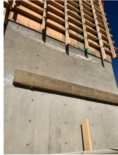
Ledger Board Install on Elevator Shaft Wall
