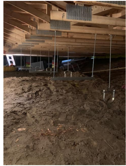
Plumbing Line Hangers Install In Crawlspace -East side
