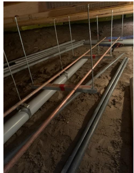
Sanitary and Domestic Water Lines with Hangers in Crawlspace – West Side
